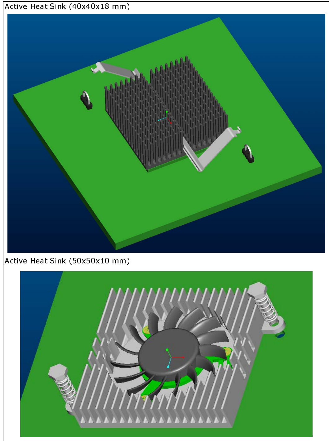
Figure 4. Intel® 413808 and 413812 SAS/SATA I/O controllers Extruded Heat sink (reference only)
