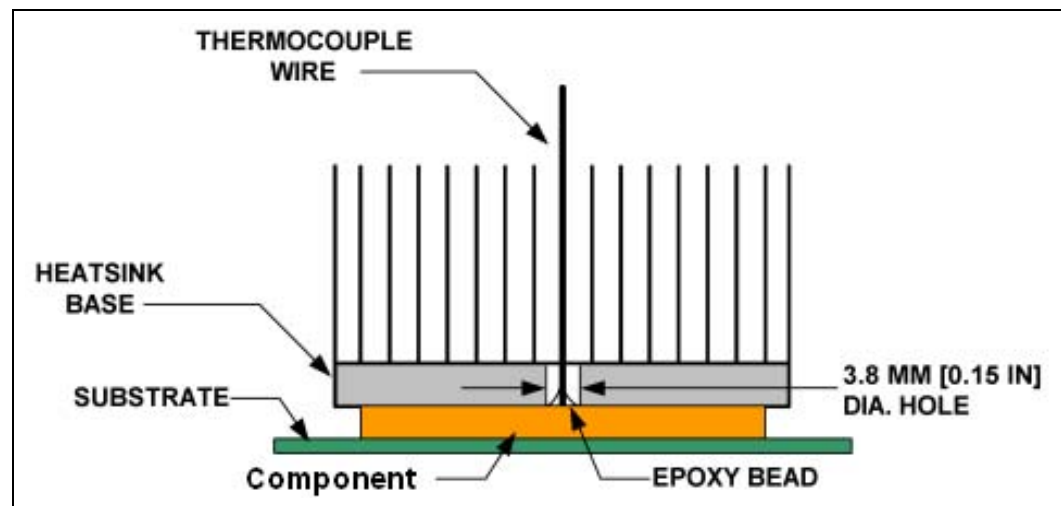
Figure 7. Technique for Measuring T case with 90° Angle Attachment
