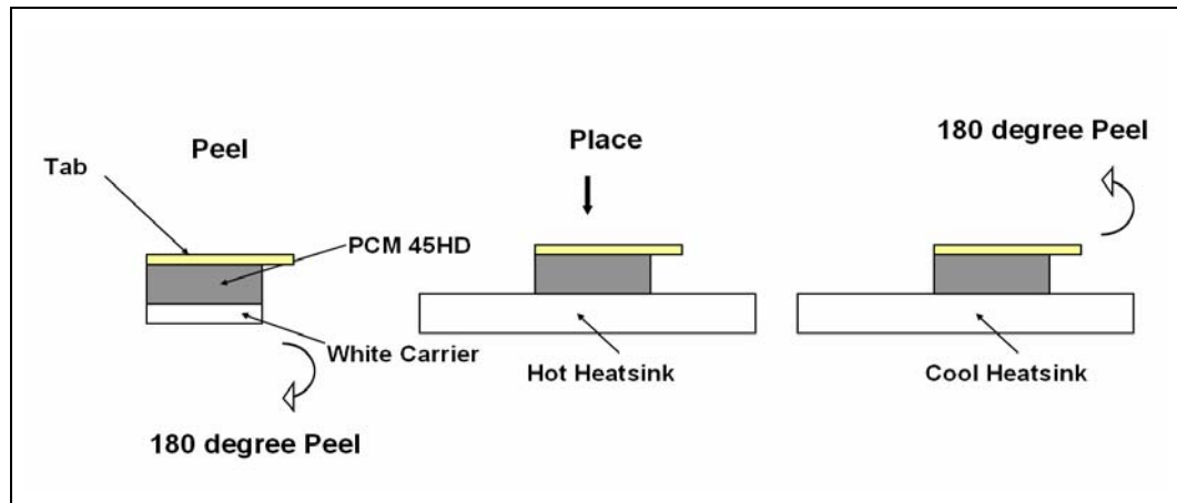
Figure 6. Completing the Attach Process
