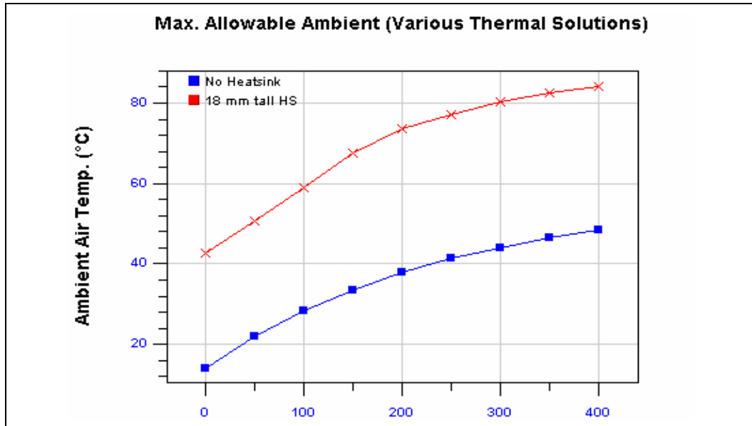
Figure 2. Maximum Allowable Ambient Temperature vs. Air Flow
