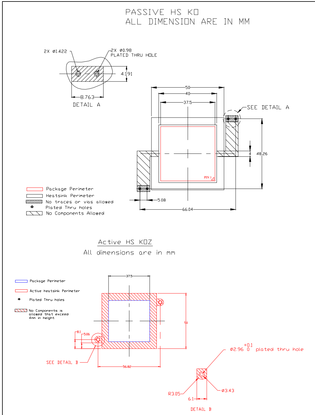
Figure 3. Intel® 413808 and 413812 SAS/SATA I/O controllers Heat Sink Keep-out Restriction
