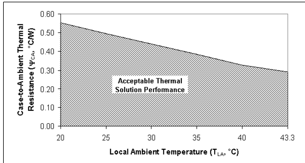
Figure 11. Thermal Resistance Values for Various Operating Temperatures
