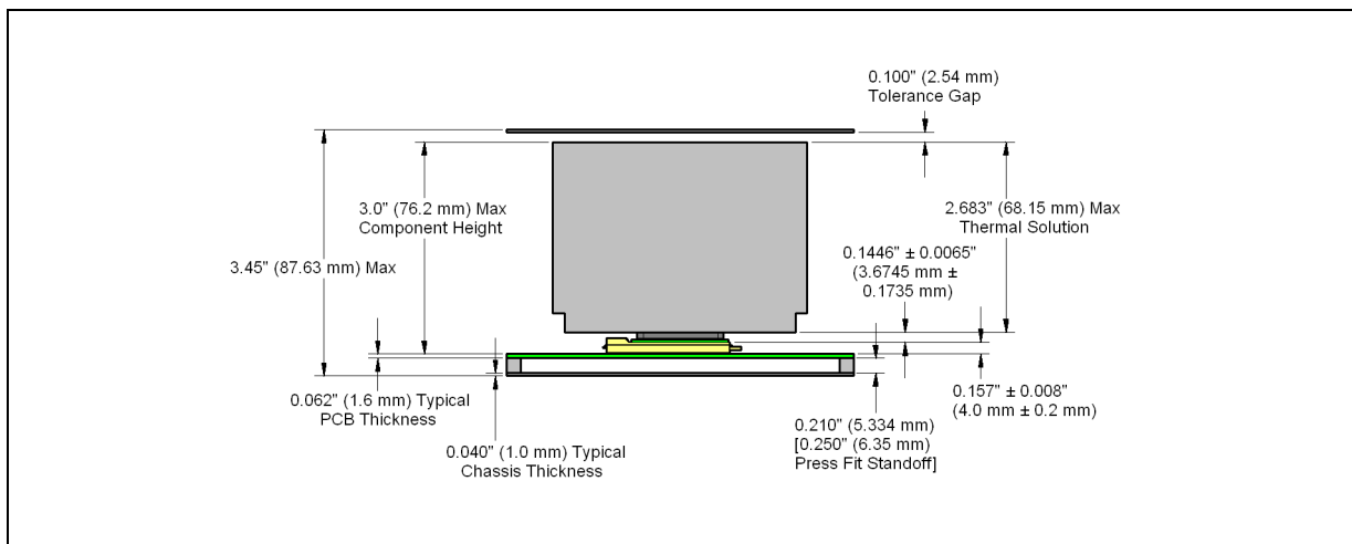
Figure 13. 2U Thermal Solution Z-Height Constraints
