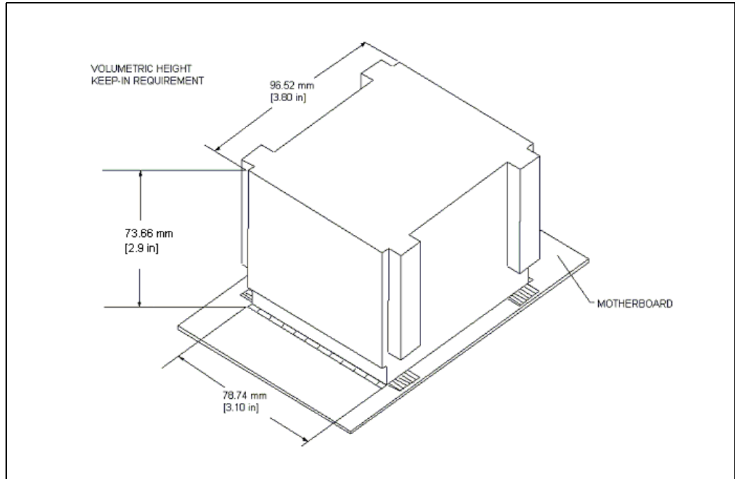
Figure 5. Volumetric Constraint for ATX/Desktop Form Factor Enabling Components
