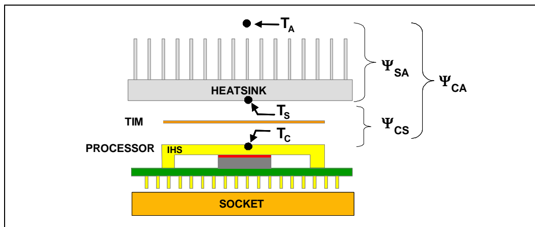
Figure 9. Processor Thermal Characterization Parameter Relationships
