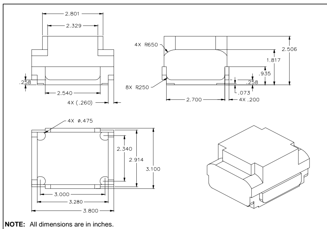
Figure 8. Heatsink, Fan, and Shroud Assembly Volumetric Constraint, ATX Form Factor
