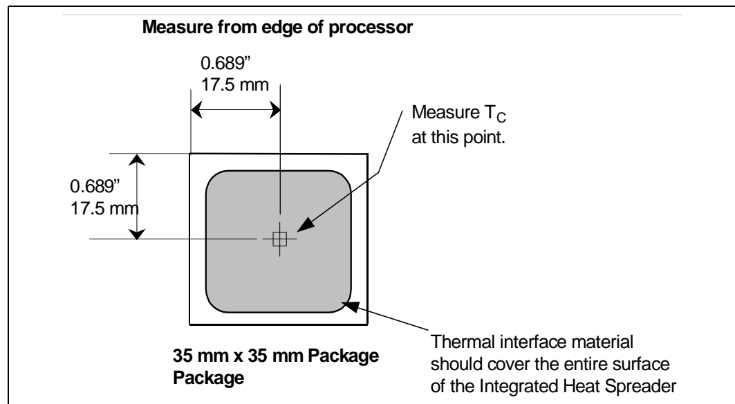
Figure 10. Processor IHS Temperature Measurement Location
