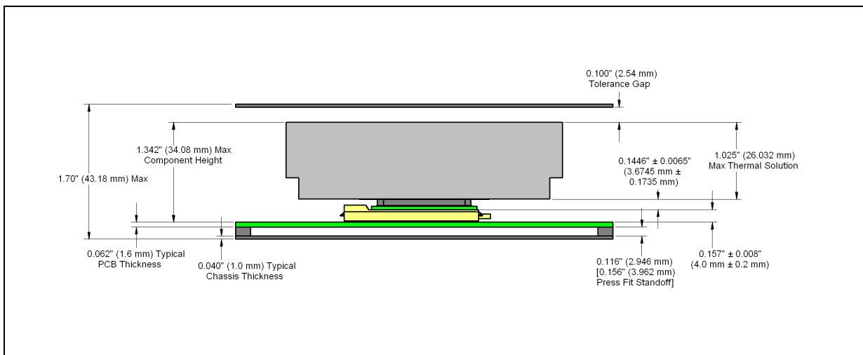
Figure 12. 1U Thermal Solution Z-Height Constraints
