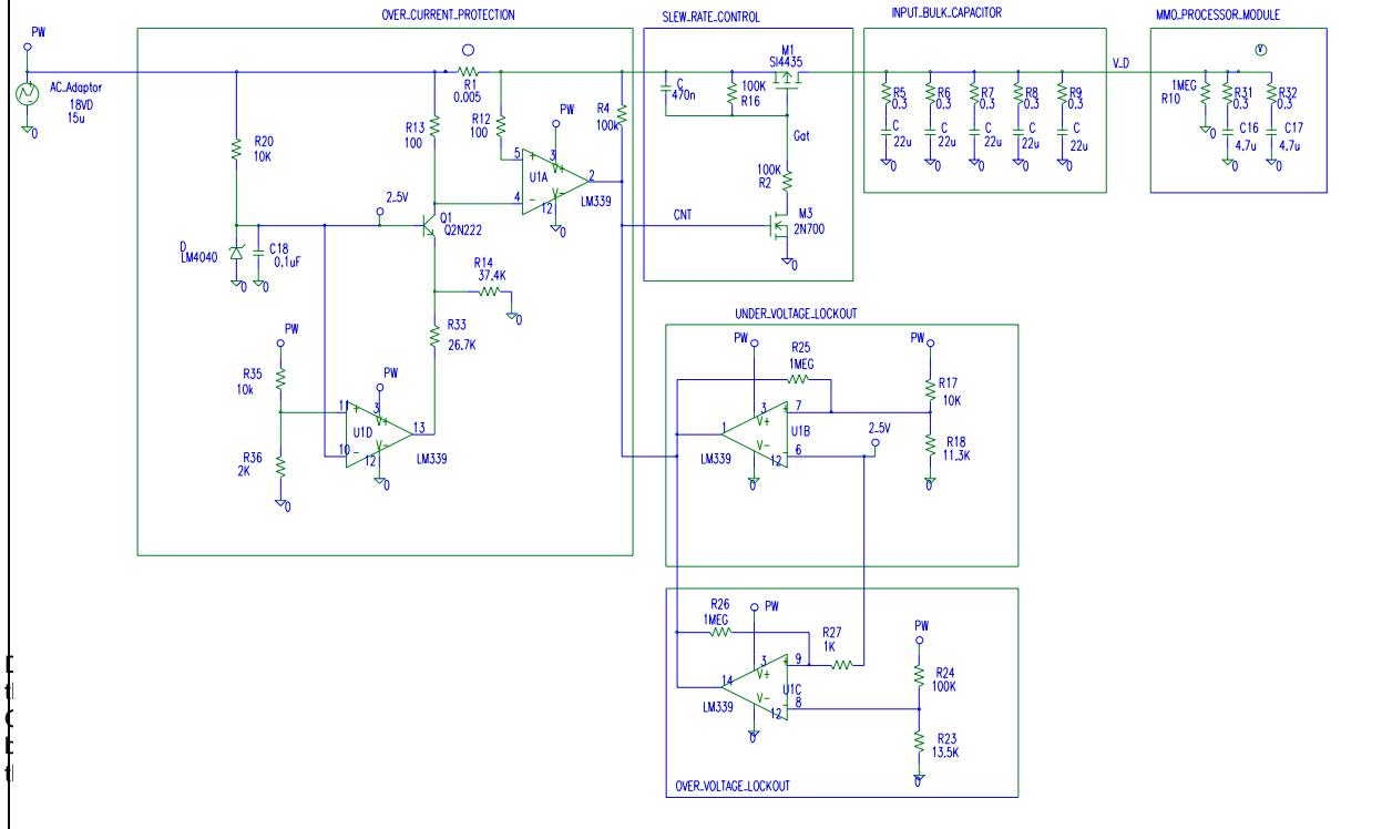
Figure 8. Overcurrent Protection Circuit
