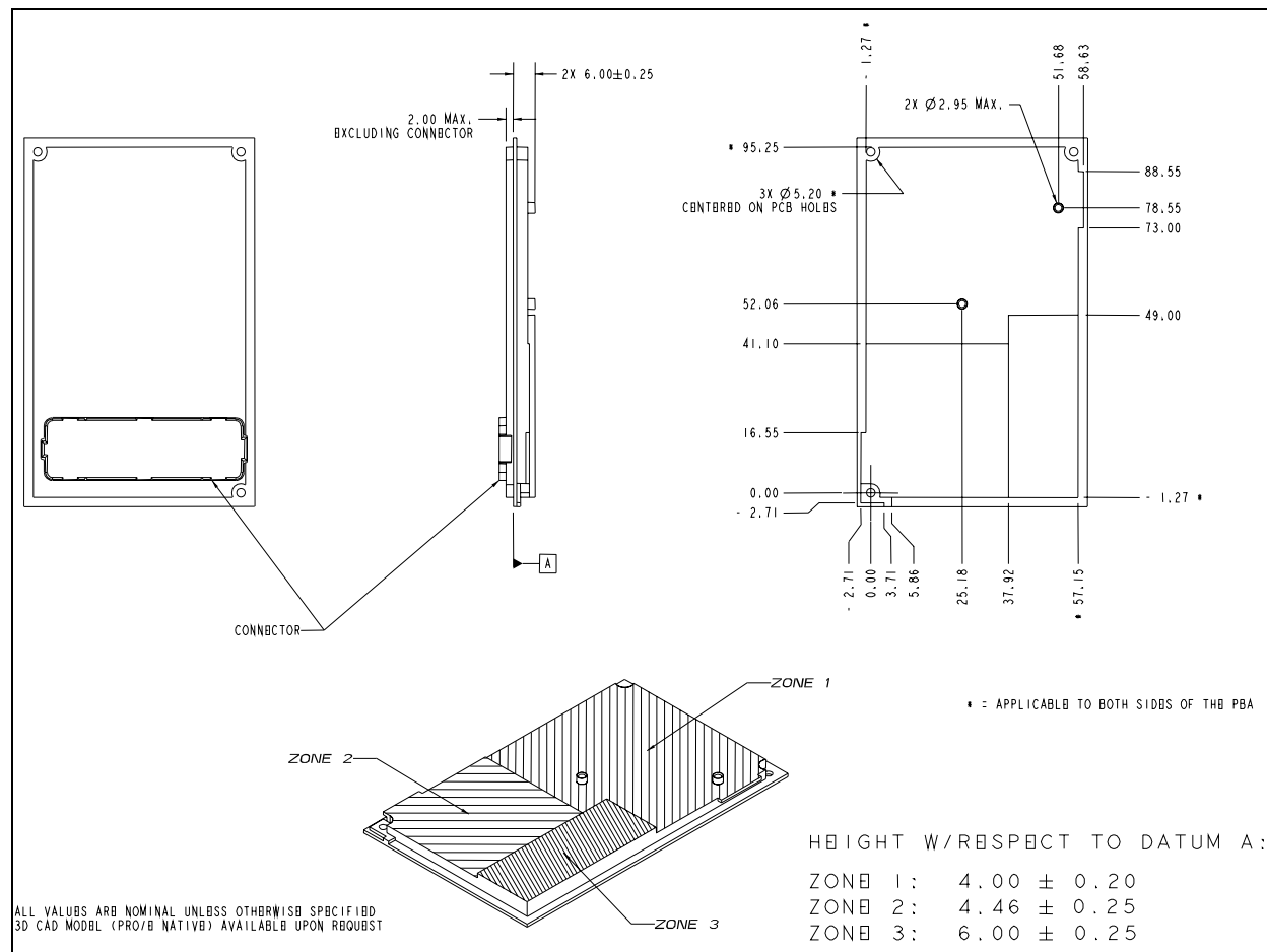
Figure 13. Keep-out Zone
