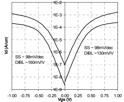
Figure 6: Sub-threshold curves
