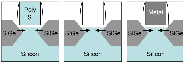
Form Transistors Remove Poly Si Deposit Metal Gate Figure 2: Increased channel strain due to RMG process flow
