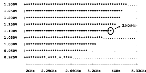
Figure 15: Voltage-frequency shmoo for 291Mb SRAM
