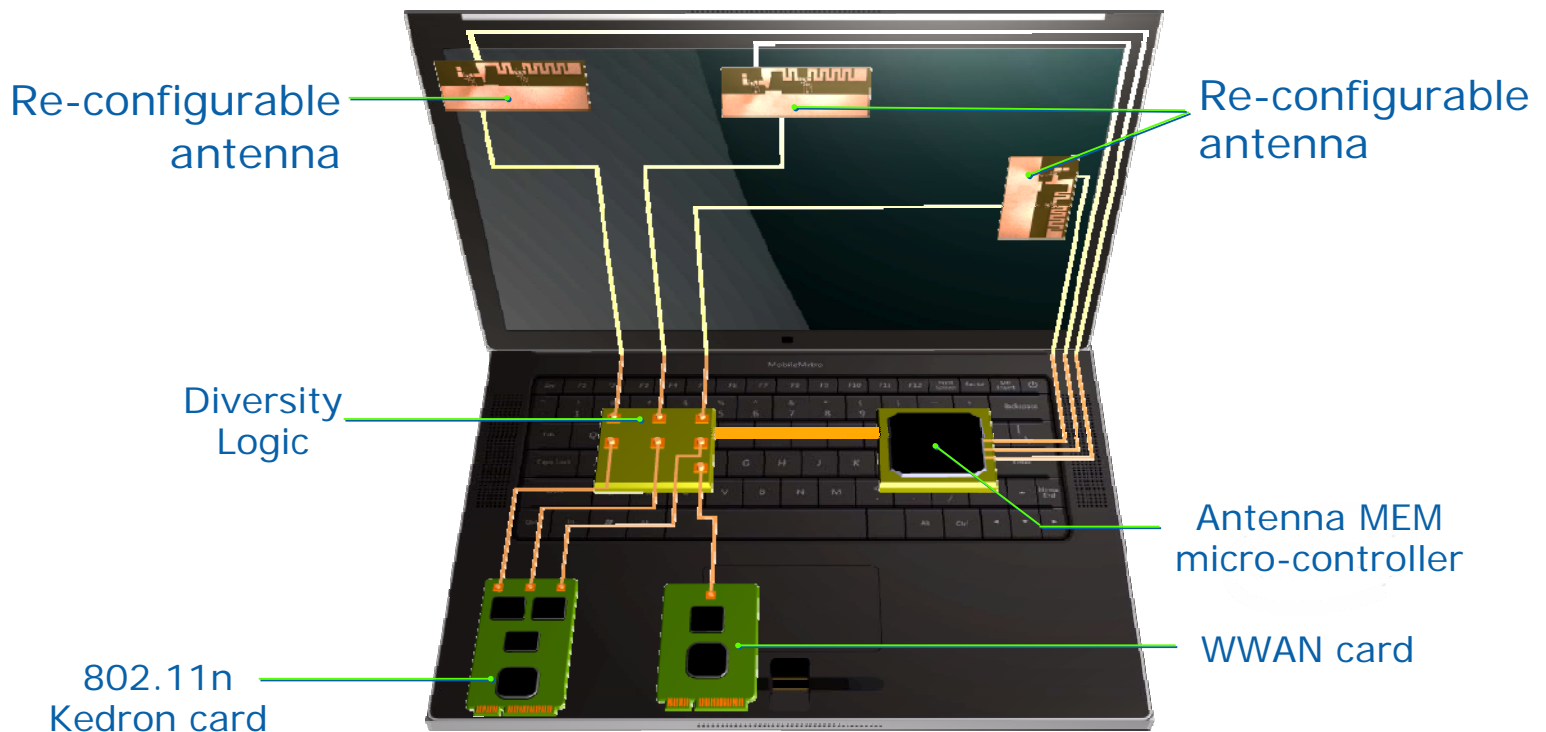
Intel Mobile Metro Concept PC Utilizing Reconfigurable Antenna and Switching System
