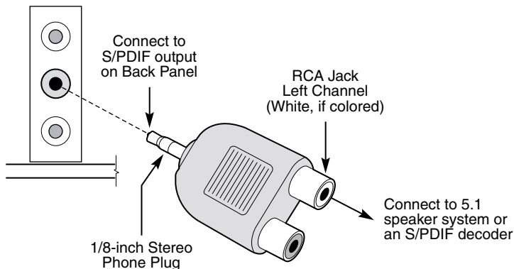
Figure 8. Adapter for S/PDIF Back Panel Connector
