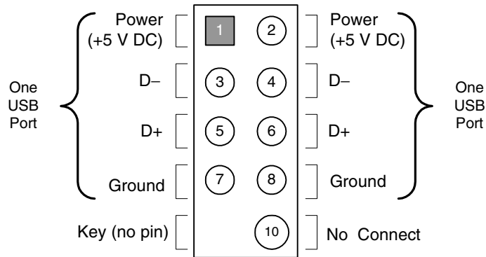
Figure 20. Connection Diagram for Front Panel USB Connectors
