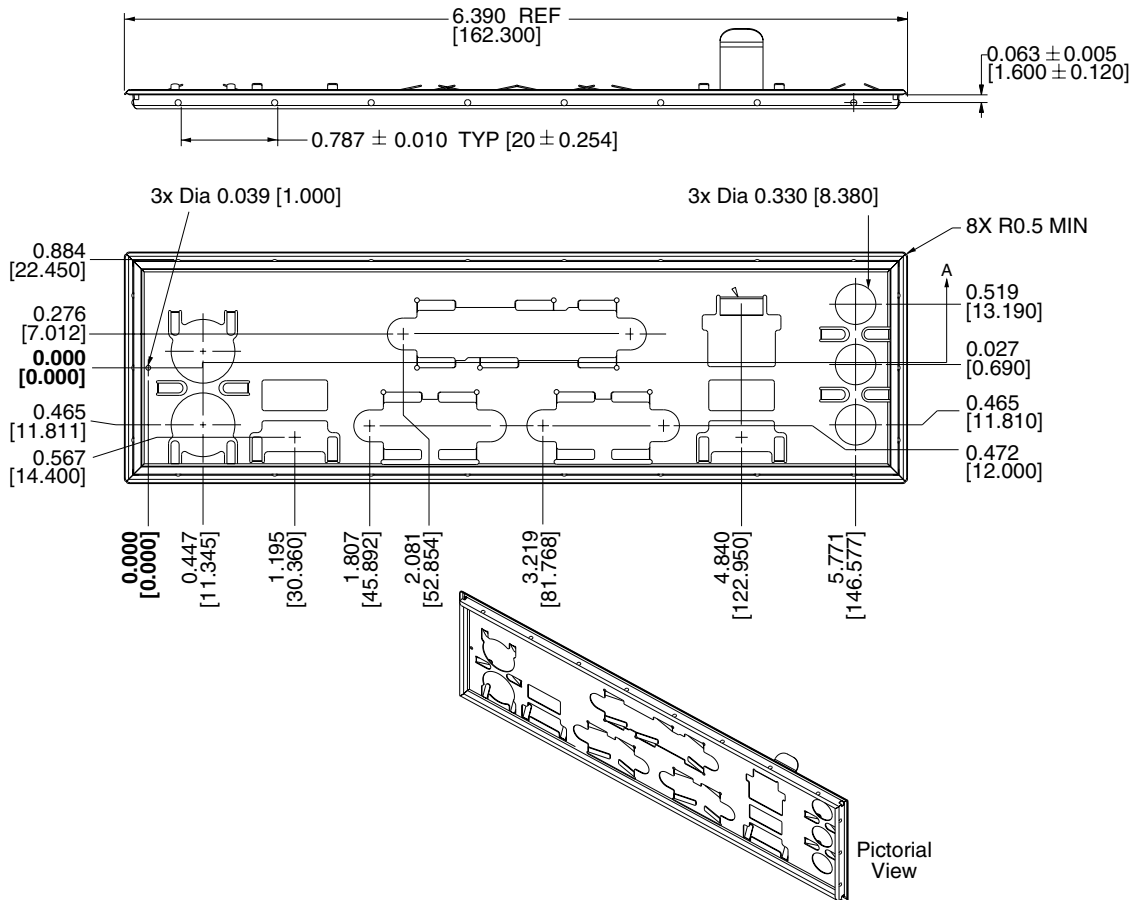
Figure 23. I/O Shield Dimensions
