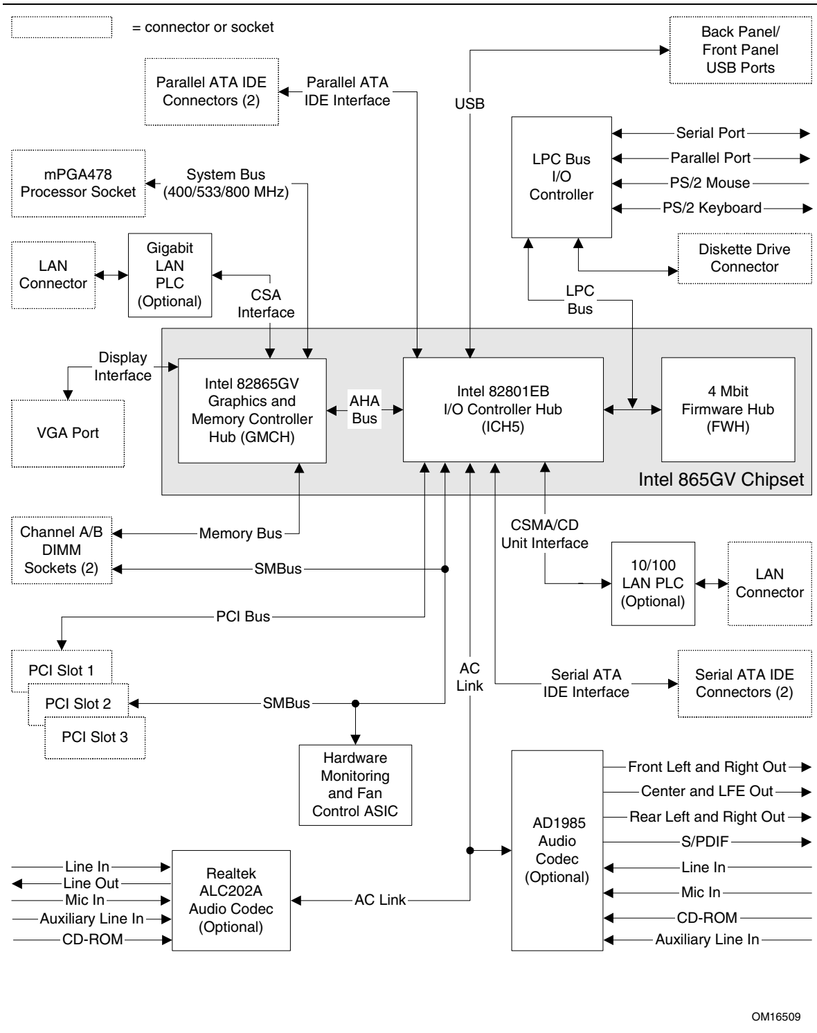
Figure 2. Block Diagram
