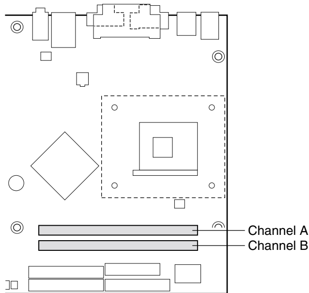
Figure 3. Memory Channel Configuration
