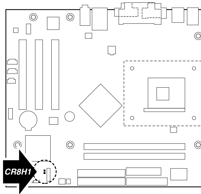
Figure 13. Location of the Standby Power Indicator LED on the D865GVHZ Board
