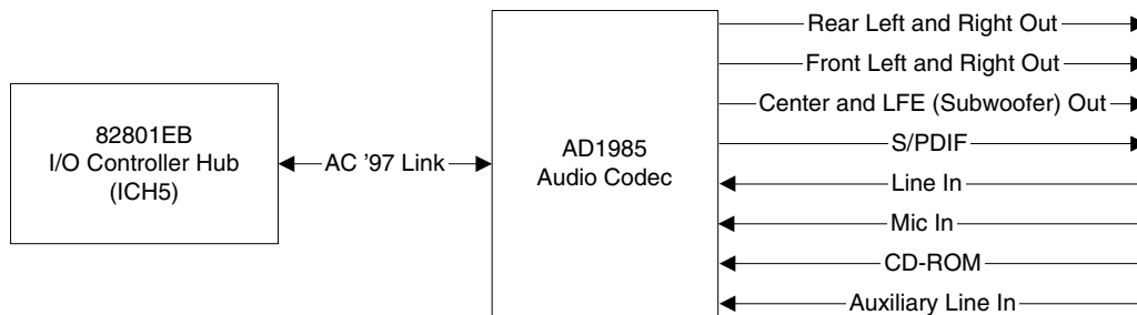
Figure 9. Flex 6 Audio Subsystem Block Diagram
