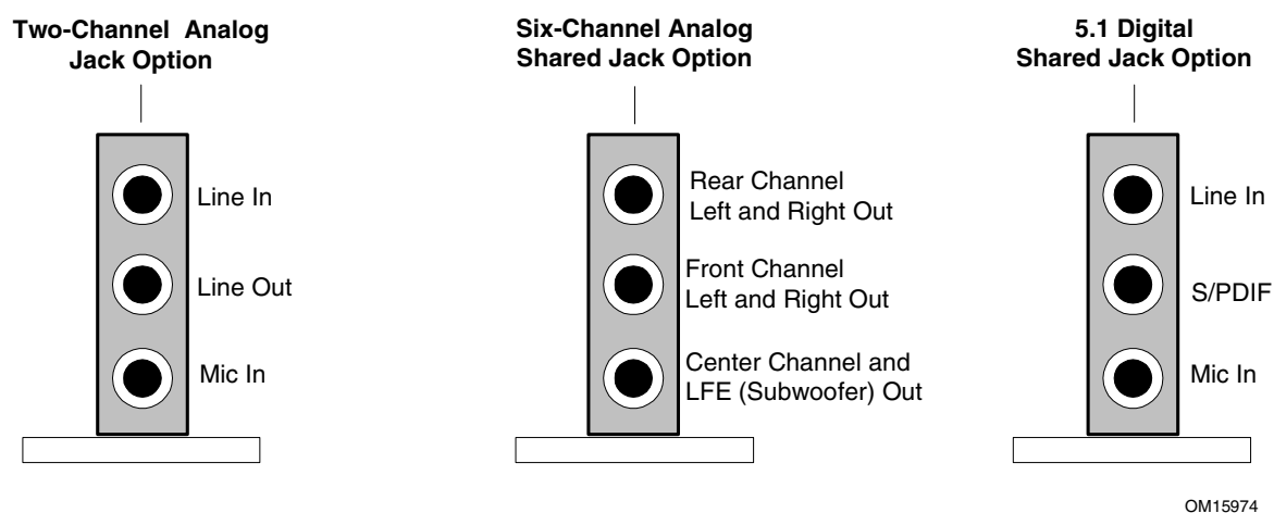
Figure 7. Back Panel Audio Connector Options for Flex 6 Audio Subsystem
