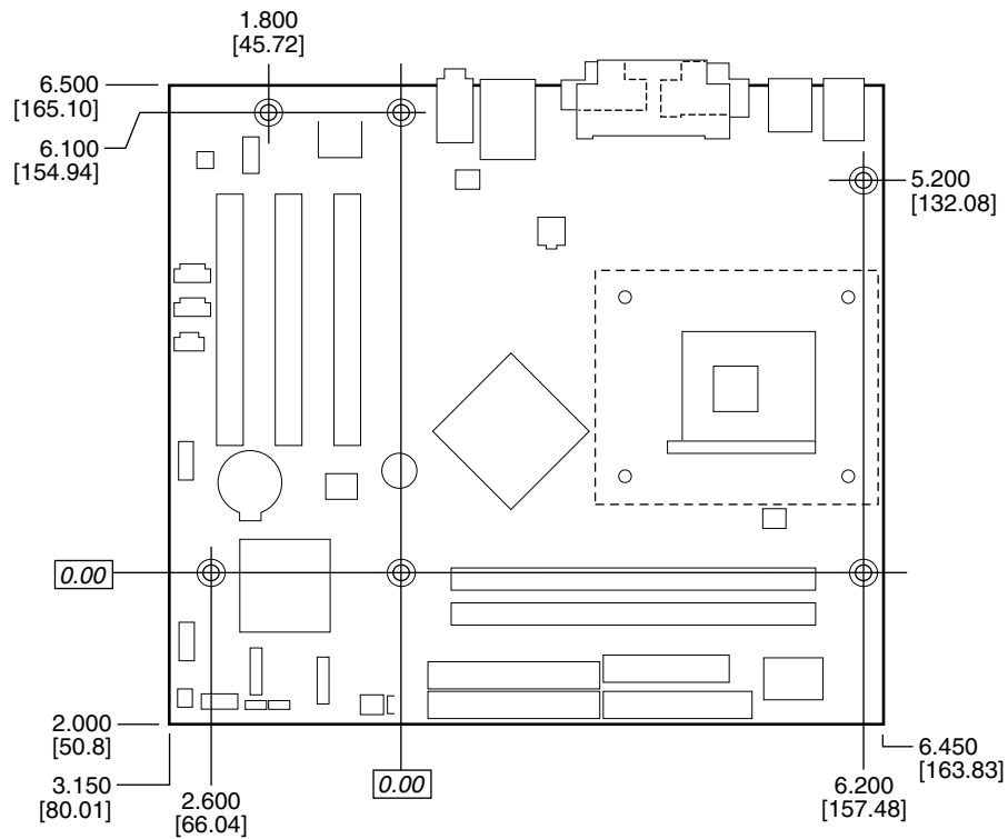
Figure 22. Desktop Board D865GVHZ Dimensions
