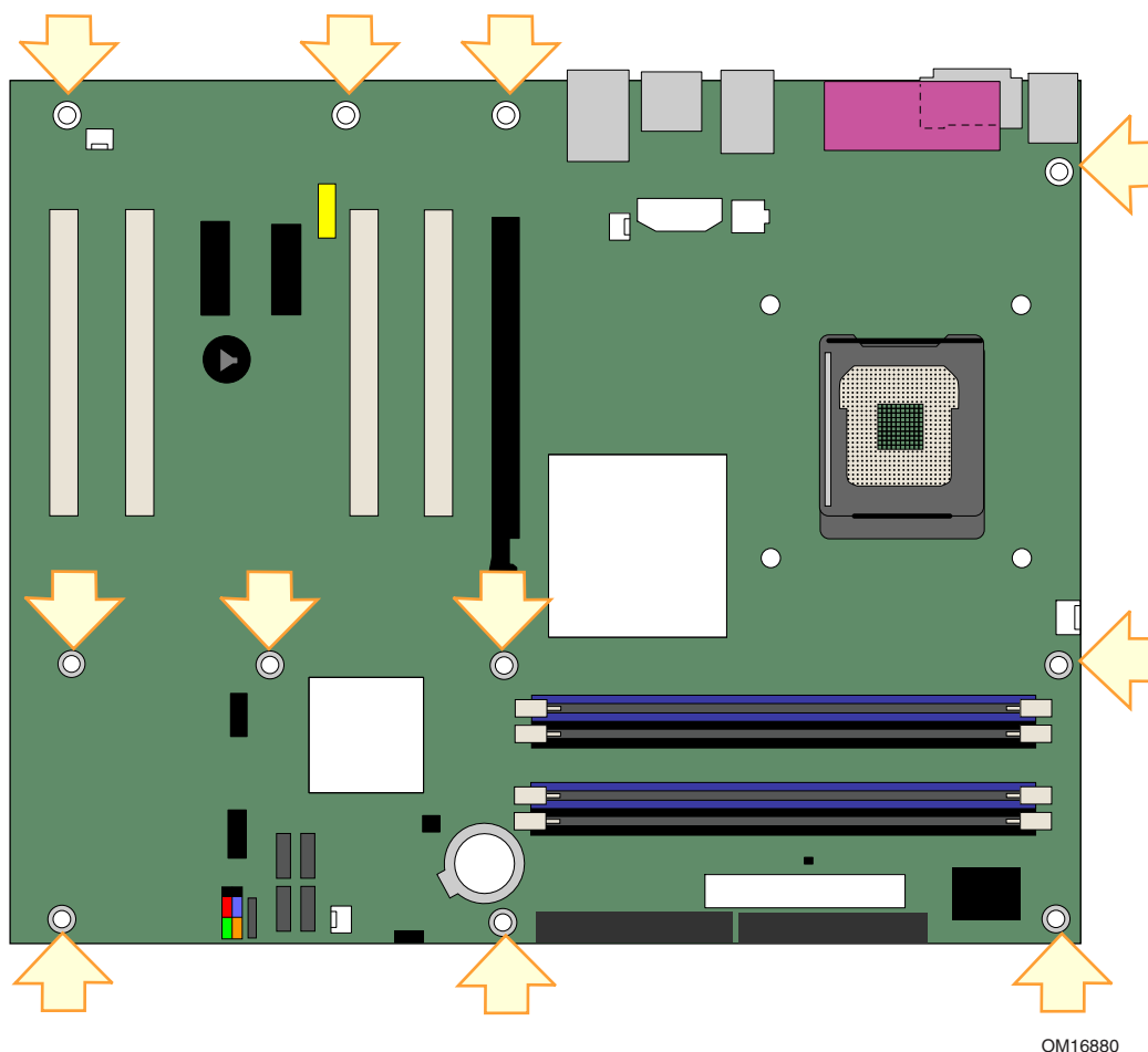
Figure 5. Desktop Board D915PGN and D915PCY Mounting Screw Hole Locations
