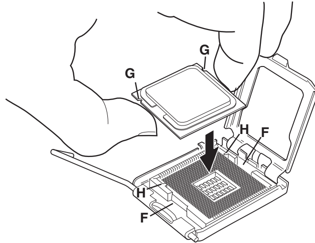
Figure 10. Install Processor
