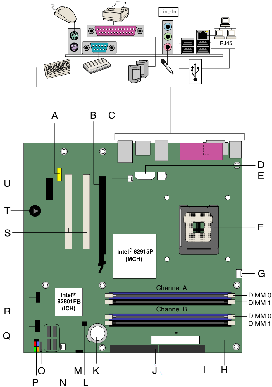
Figure 2. Intel Desktop Boards D915PSY and D915PCM Components
