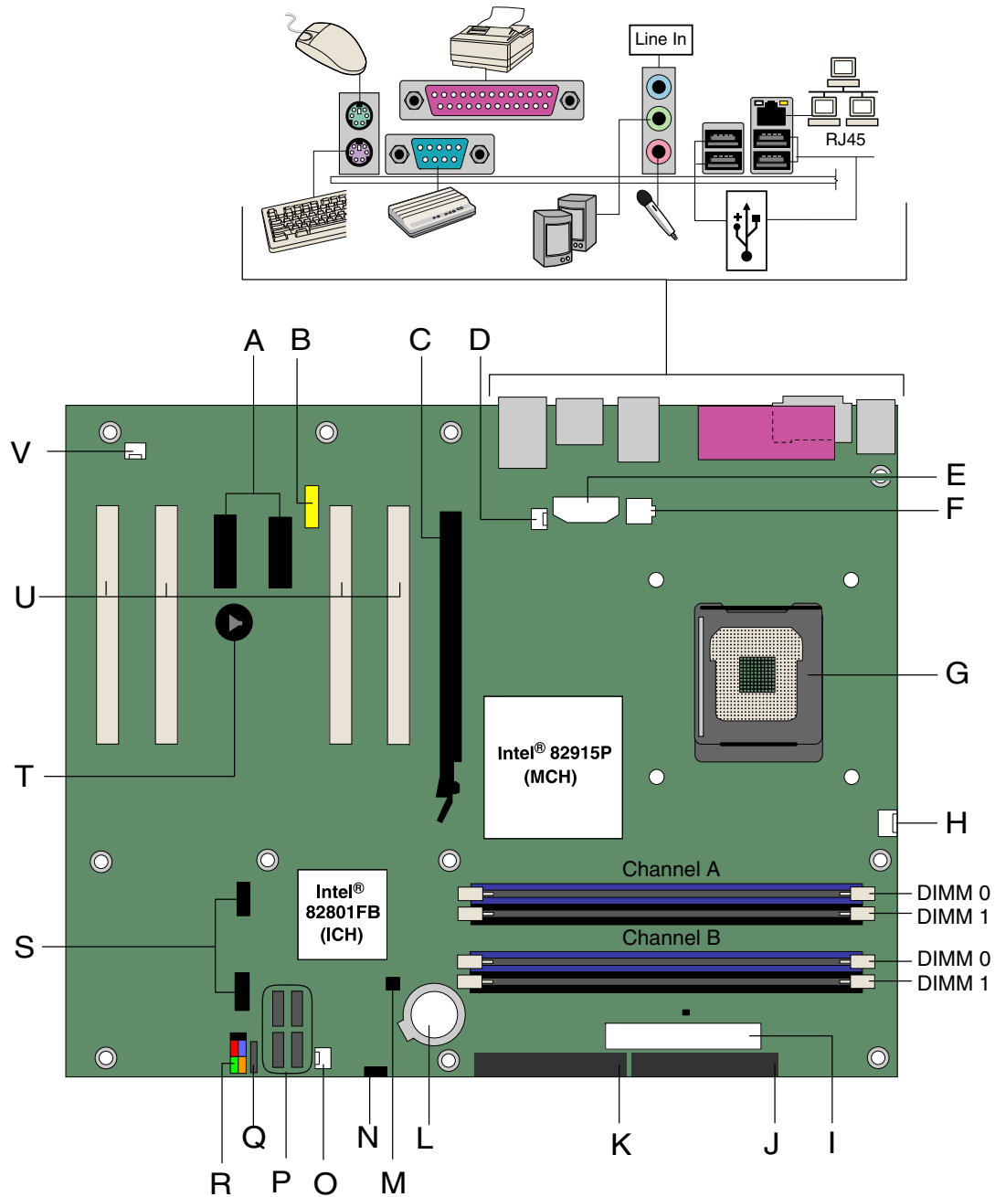
Figure 1. Desktop Boards D915PGN and D915PCY Components
