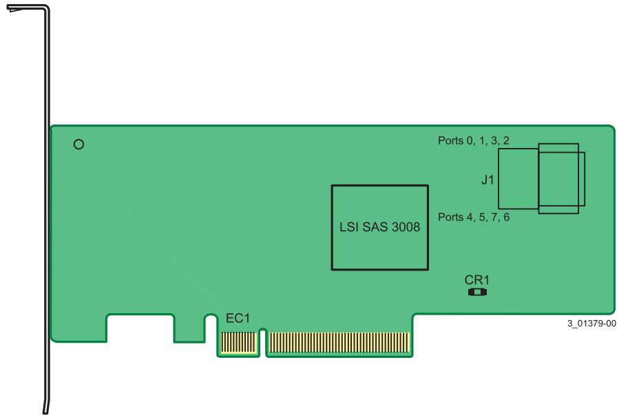
Figure 1. Server [Product Name] Board Layout
