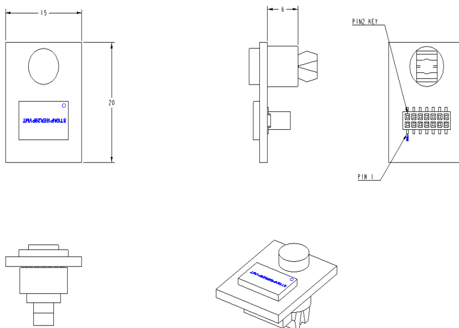
Figure 2. TPM Dimensioned Drawing
