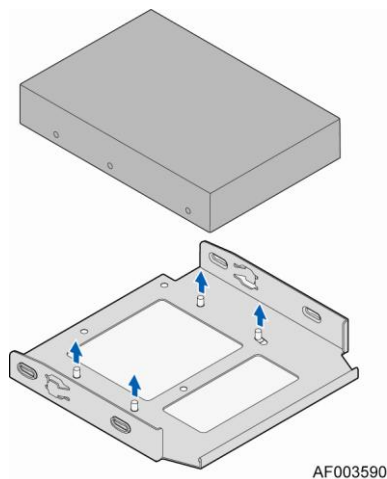
Figure 6. Fixed Drive Tray
