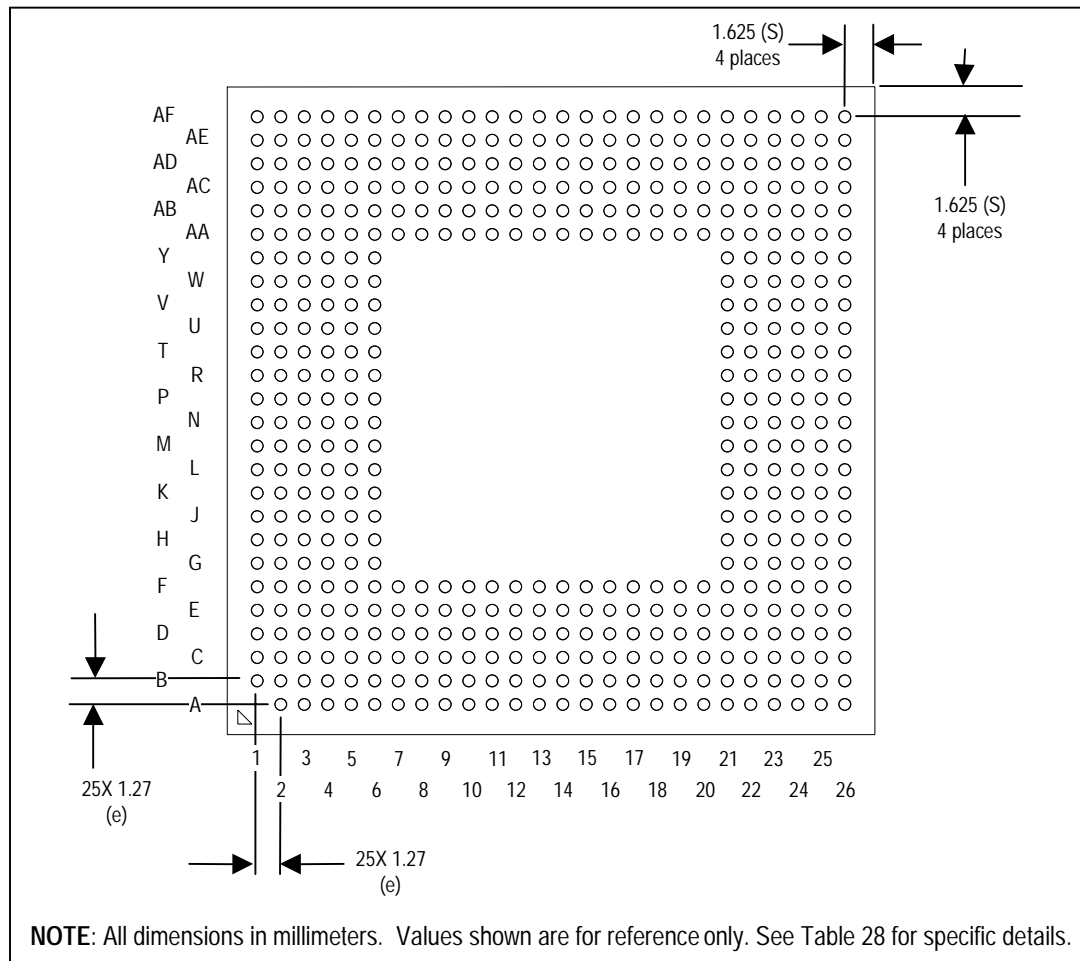
Figure 20. Micro-FCBGA Package - Bottom View
