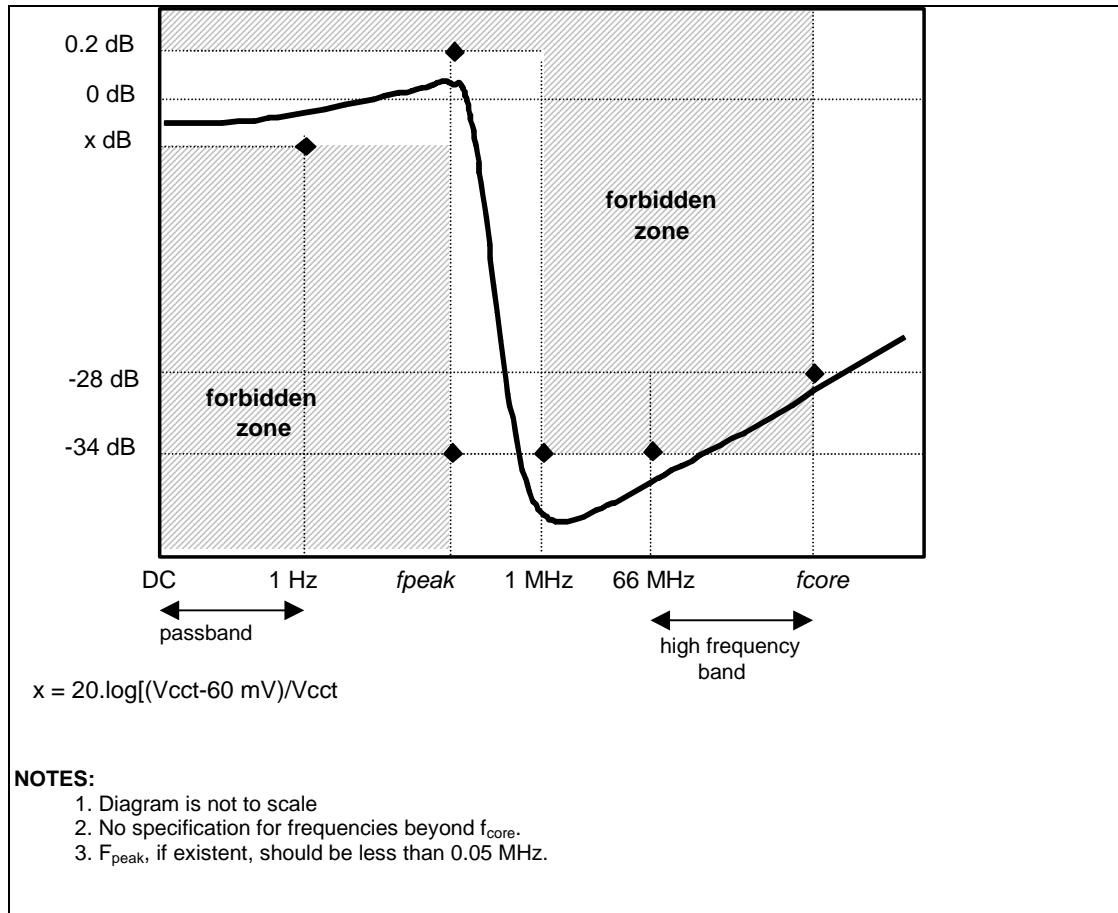
Figure 22. PLL Filter Specifications
