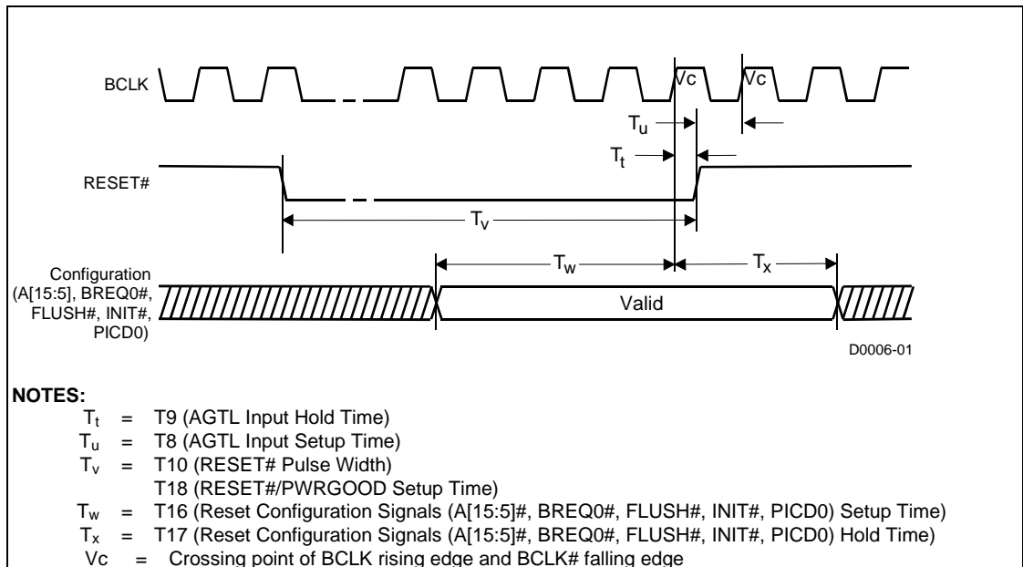
Figure 8. Cold/Warm Reset and Configuration Timings
