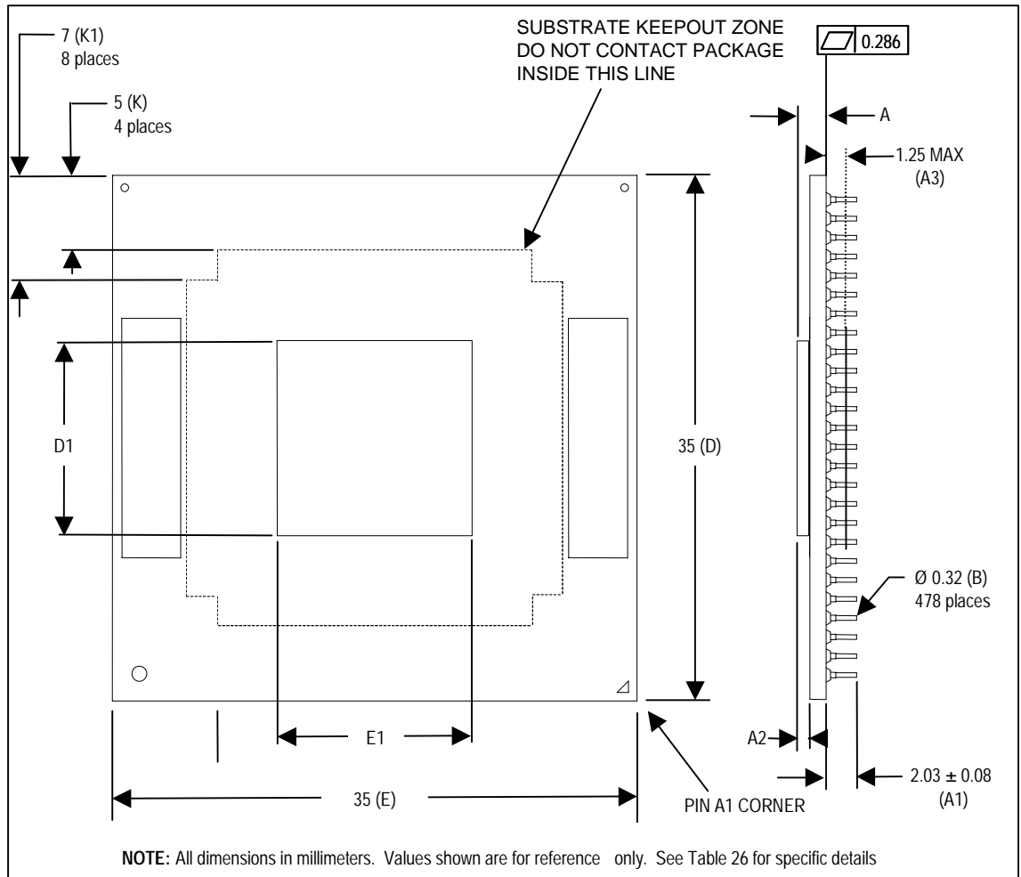
Figure 16. Socketable Micro-FCPGA Package - Top and Side View
