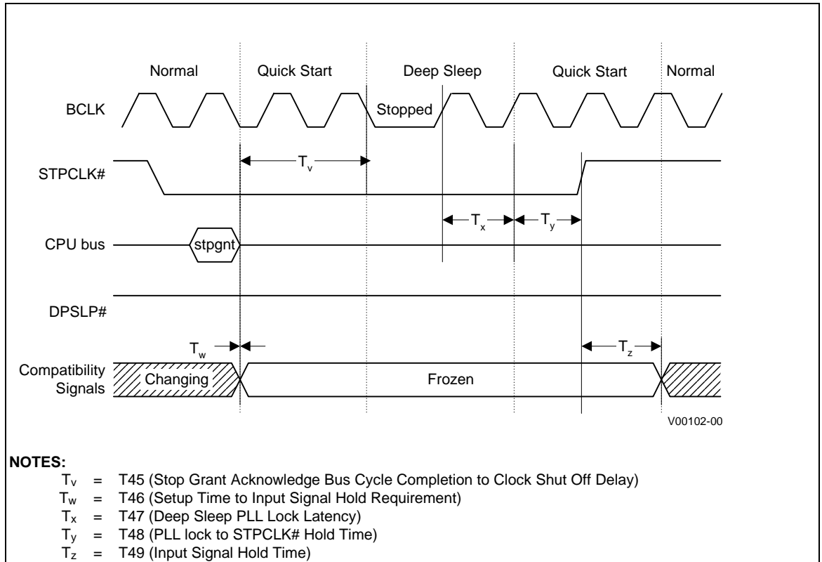
Figure 12. Quick Start/Deep Sleep Timing
