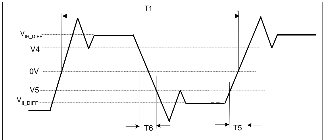
Figure 5B. BCLK/BCLK# Waveform (Differential Mode)
