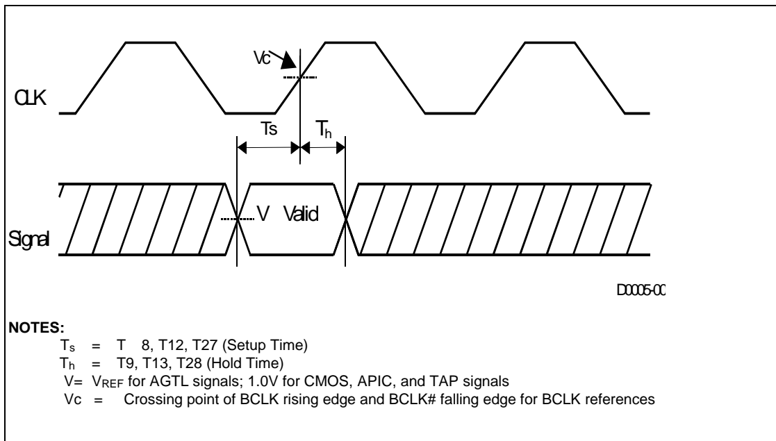
Figure 7. Setup and Hold Timings
