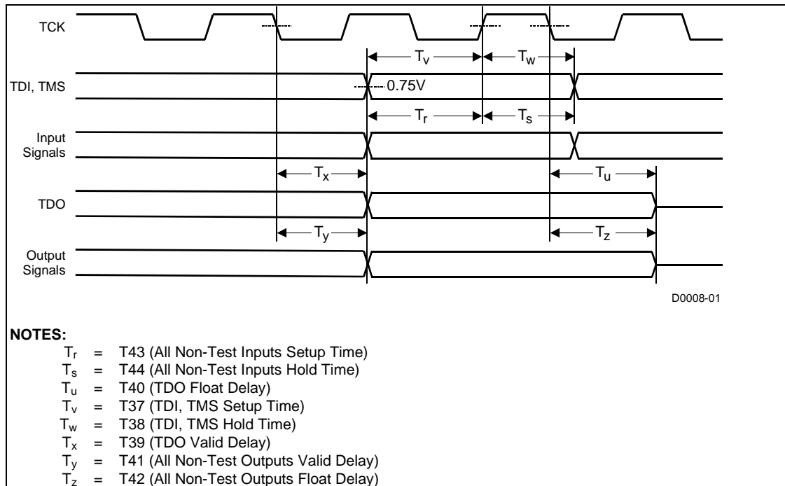
Figure 10. Test Timings (Boundary Scan)
