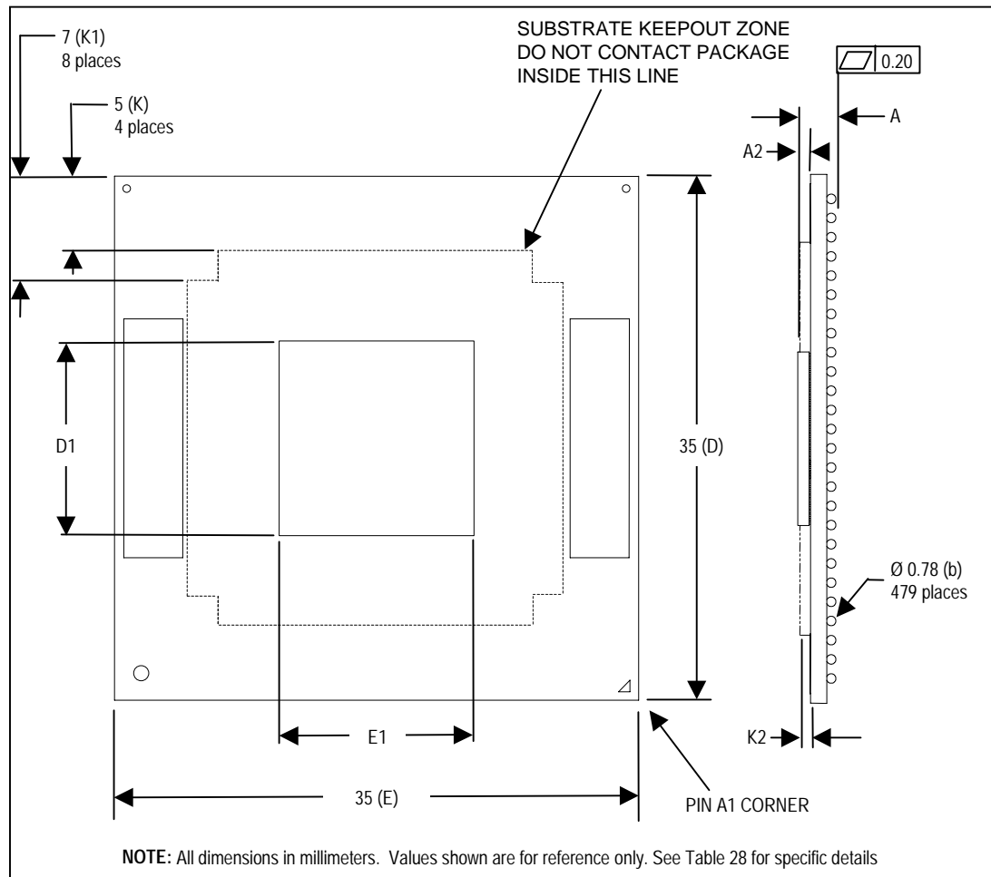
Figure 19. Micro-FCBGA Package – Top and Side Views
