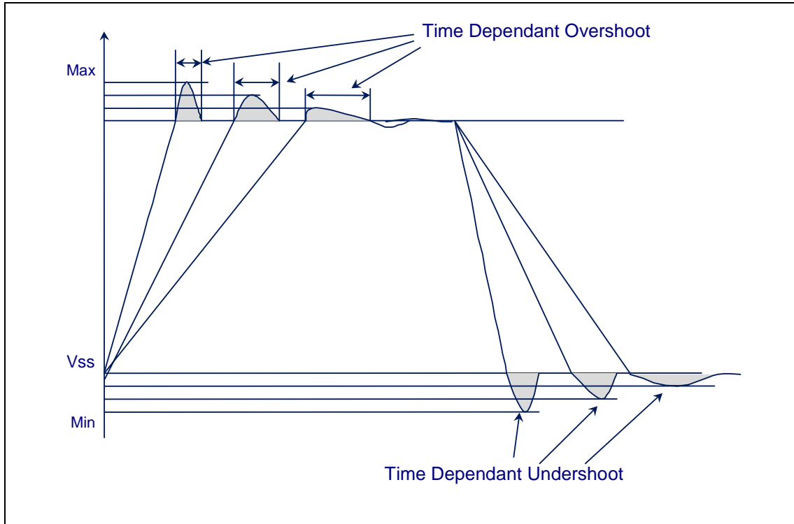
Figure 14. Maximum Acceptable Overshoot/Undershoot Waveform
