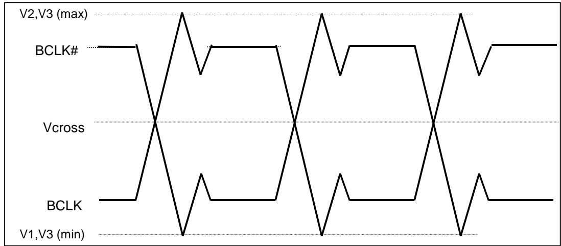
Figure 5A. BCLK/BCLK# Waveforms (Common Mode)
