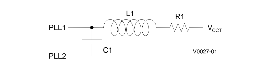
Figure 3. PLL RLC Filter
