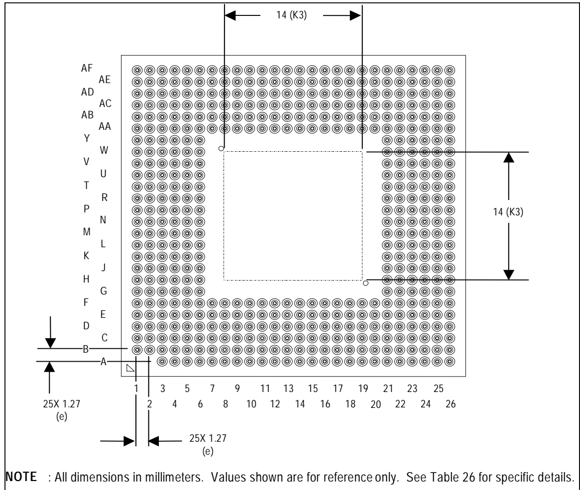
Figure 17. Socketable Micro-FCPGA Package - Bottom View
