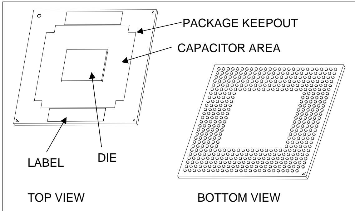
Figure 18. Micro-FCBGA Package – Top and Bottom Isometric Views
