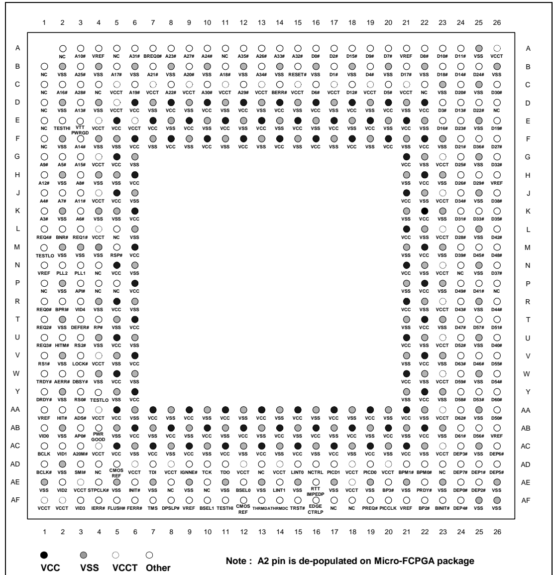
Figure 21. Pin/Ball Map - Top View
