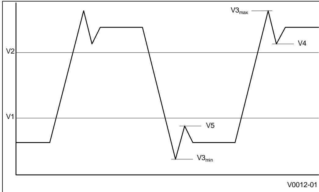
Figure 13. BCLK/PICCLK Generic Clock Waveform
