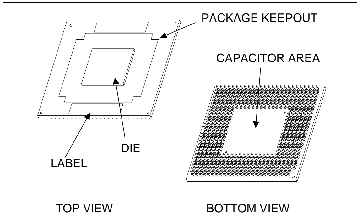
Figure 15. Socketable Micro-FCPGA Package - Top and Bottom Isometric Views
