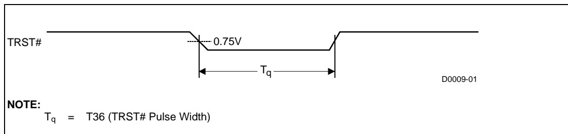
Figure 11. Test Reset Timings
