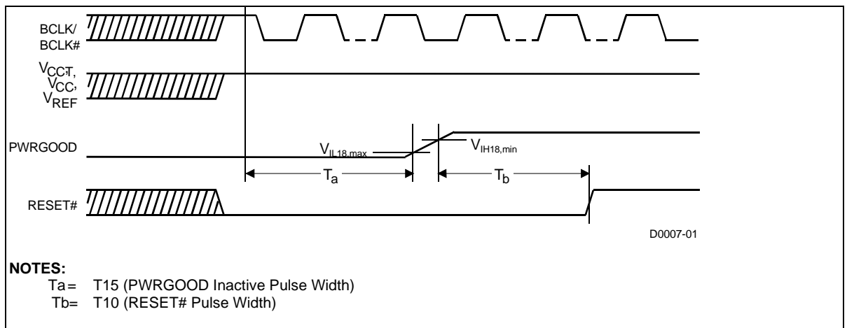
Figure 9. Power-on Reset Timings
