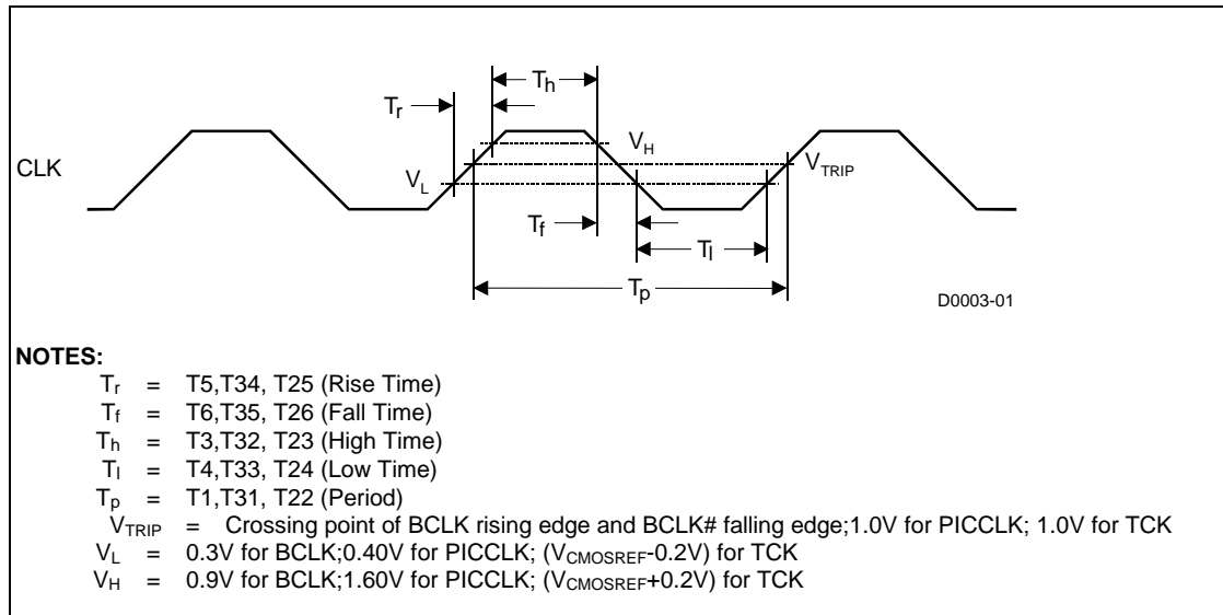
Figure 4. PICCLK/TCK Generic Clock Timing Waveform
