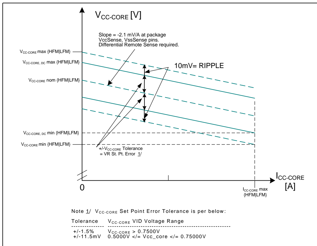
Figure 3. Active V_{CC} and I_{CC} Loadline for Pentium Processors
