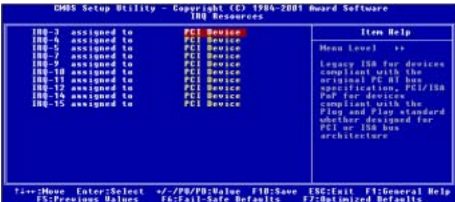
Abb. 3-8B. IRQ-Ressourcen - Setupmenü
