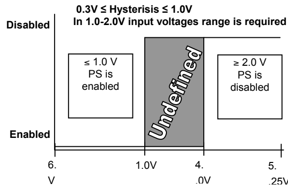
Figure 25. PSON# Required Signal Characteristics
