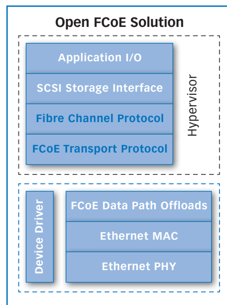
Figure 2. Overview of Open Fibre Channel over Ethernet initiator solution.
