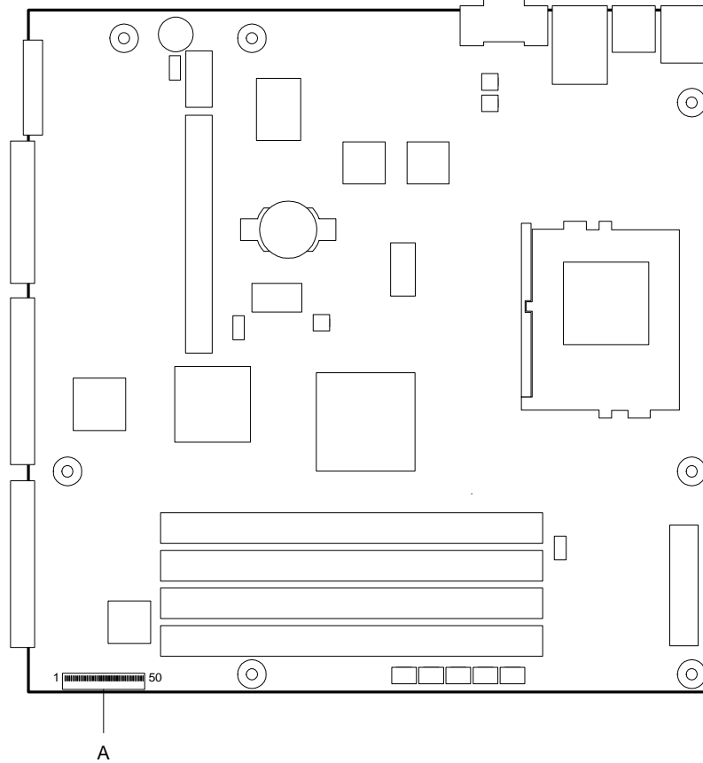
Figure 14: Front panel connector
