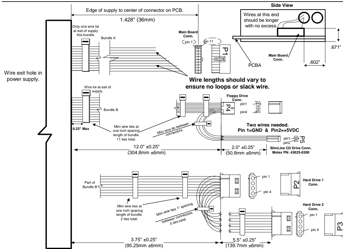
Figure 5: DC output wire harness
