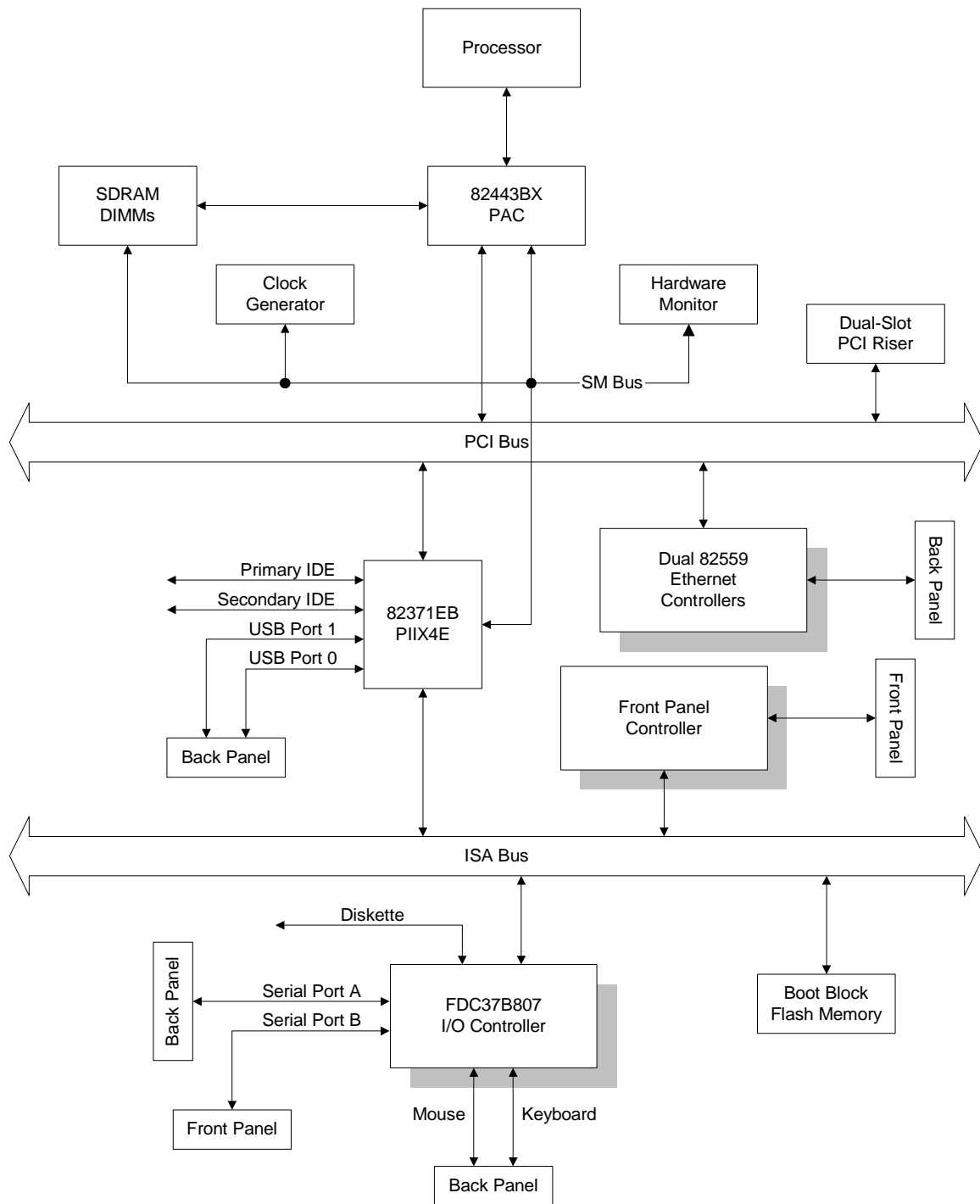
Figure 8 is a block diagram of the ISP1100 motherboard.
