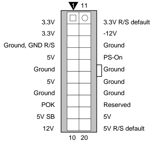
Figure 4: DC connector pinout
