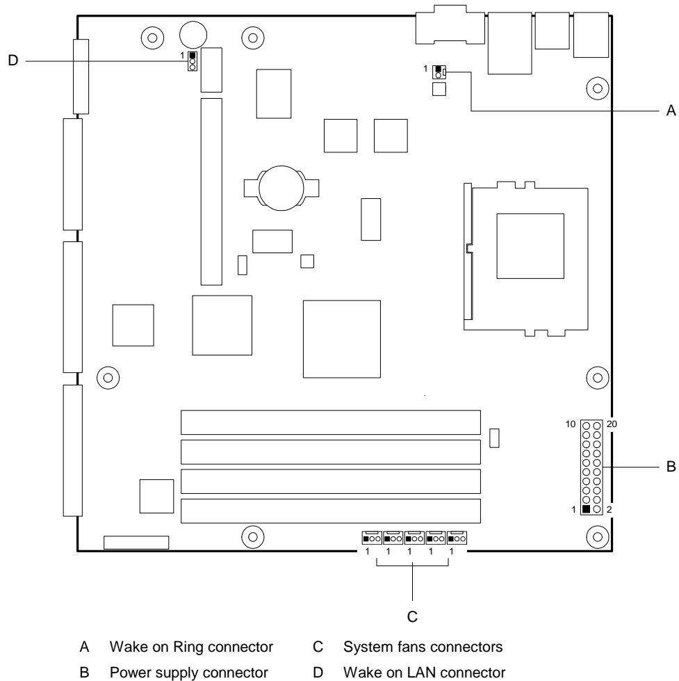
Figure 12: Hardware management and power connectors
