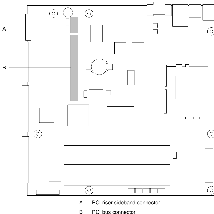
Figure 13: PCI riser sideband and PCI bus connectors
