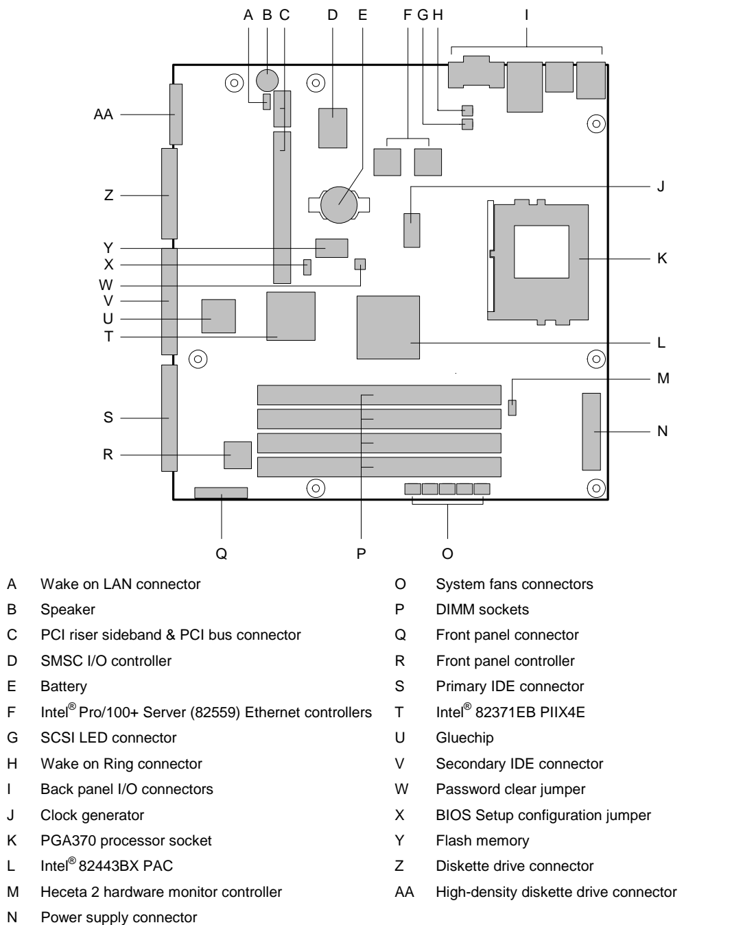
Figure 7: ISP1100 motherboard components
