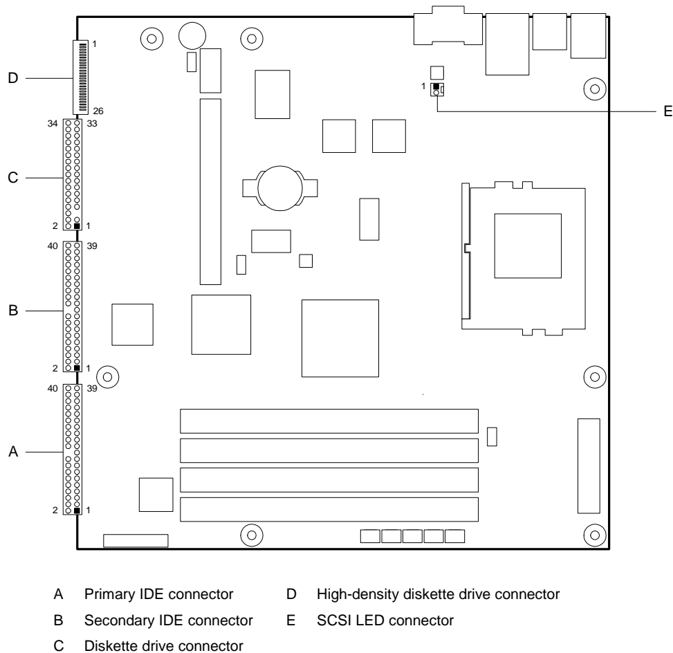
Figure 11: Peripheral connectors
