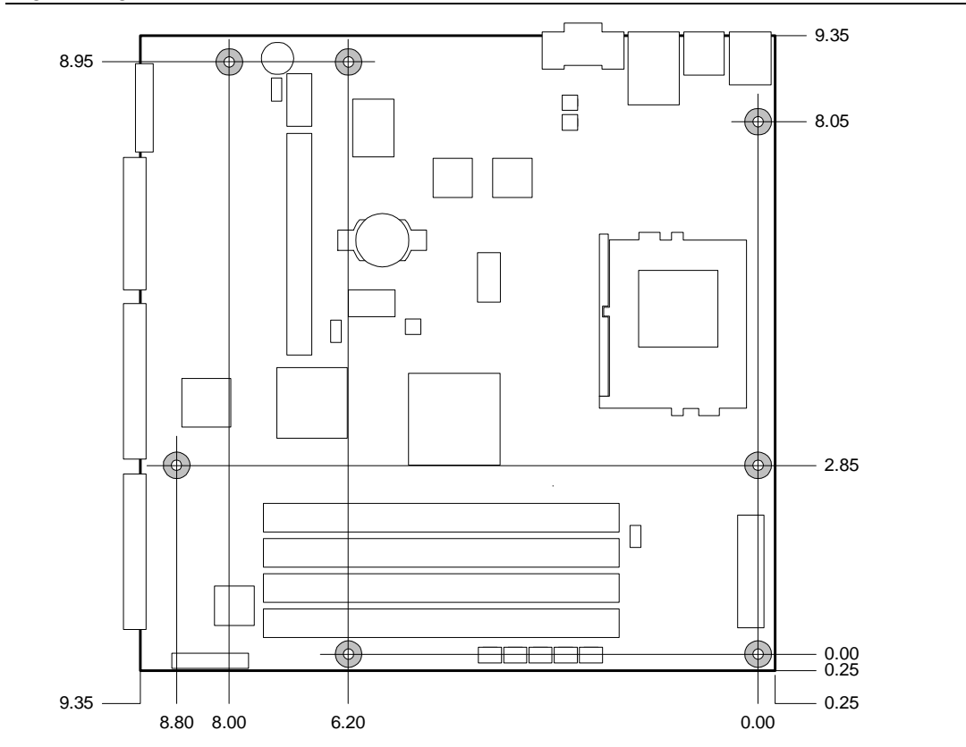
Figure 16: ISP1100 motherboard dimensions
