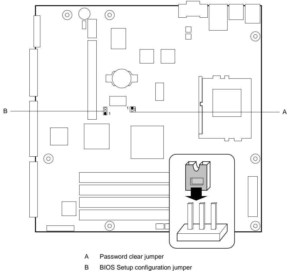
Figure 15: BIOS Setup configuration and password override jumpers
