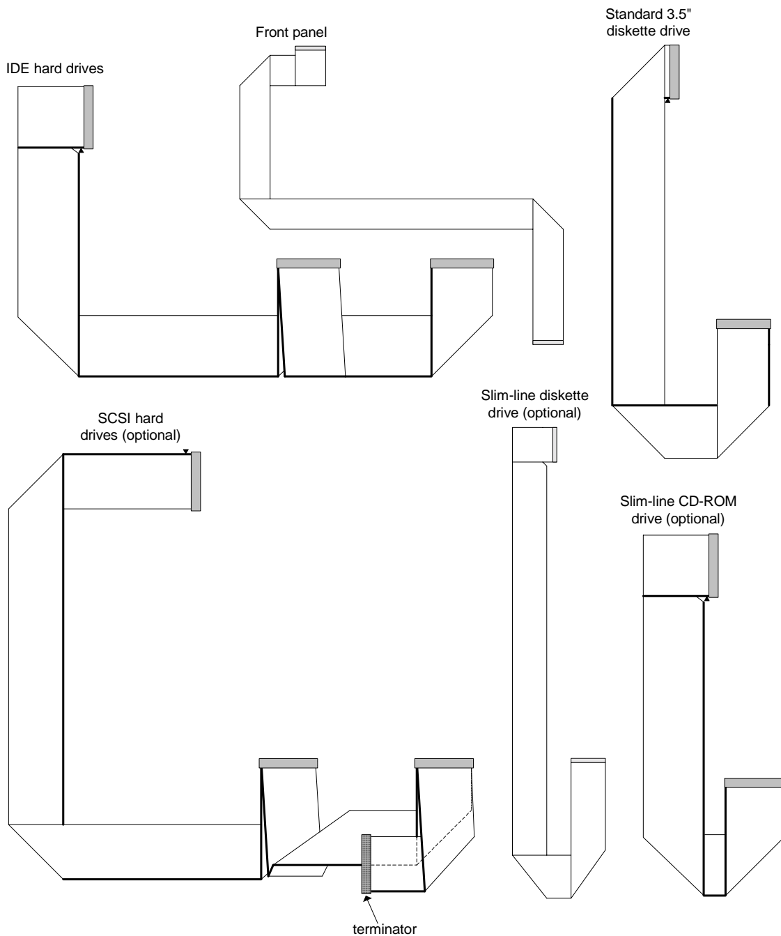
Figure 6: Internal cables
