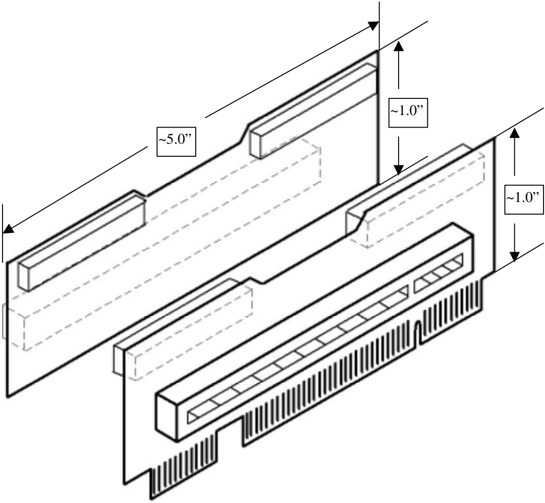
Figure 18: PCI riser board
