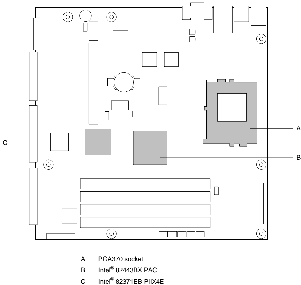
Figure 17: Thermally-sensitive components
