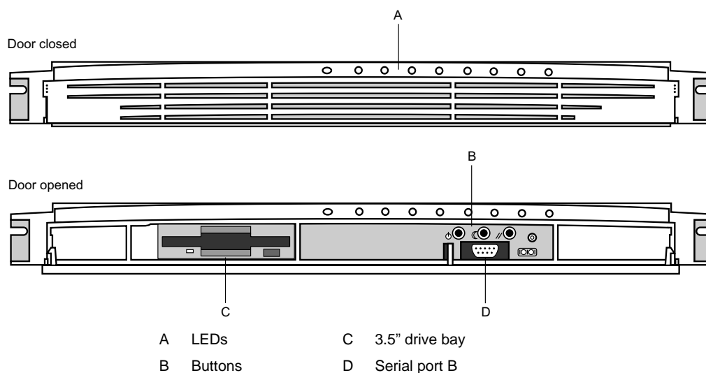
Figure 2: Front view of chassis
