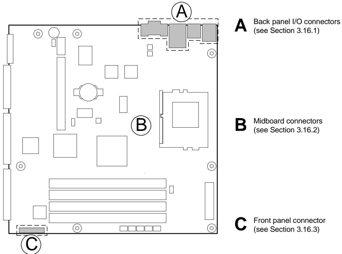
Figure 9: Connector groups
