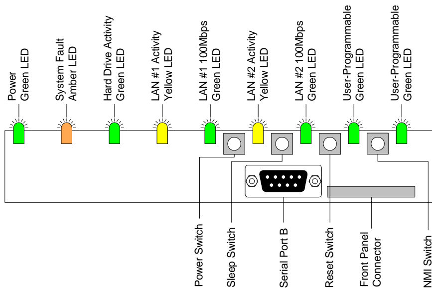
Figure 19: Front panel board
