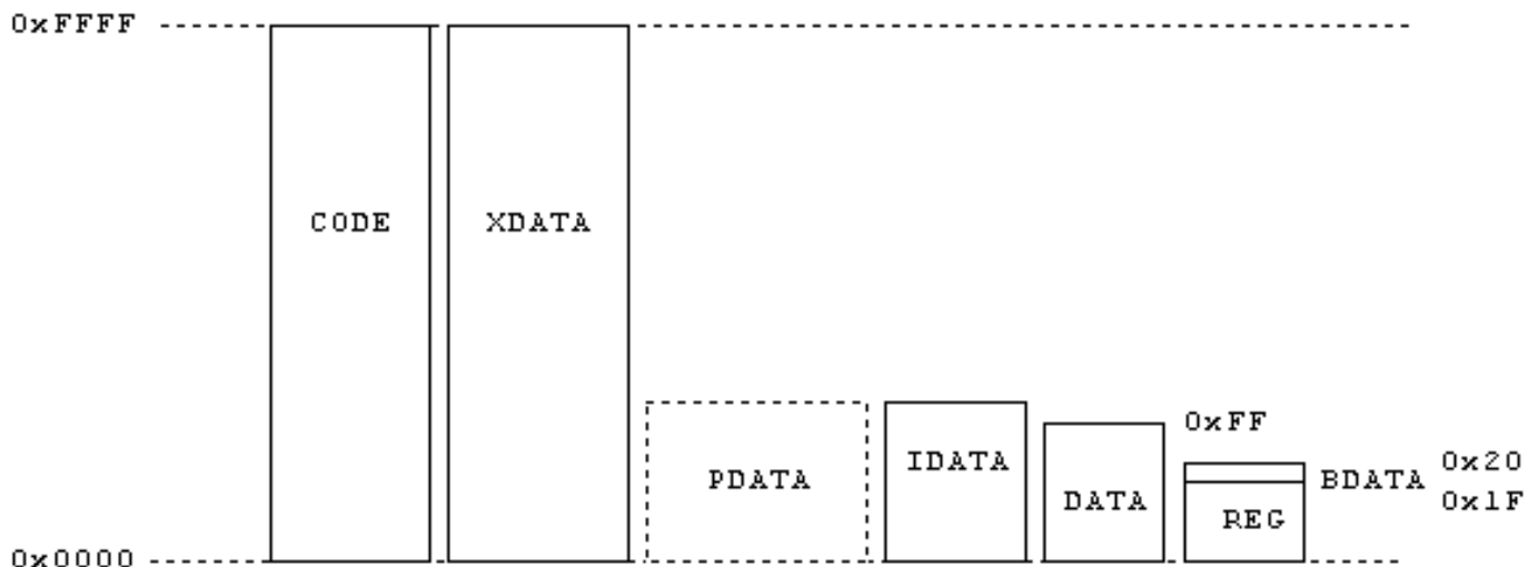
Fig.1. - The 8051's Memory Spaces.
